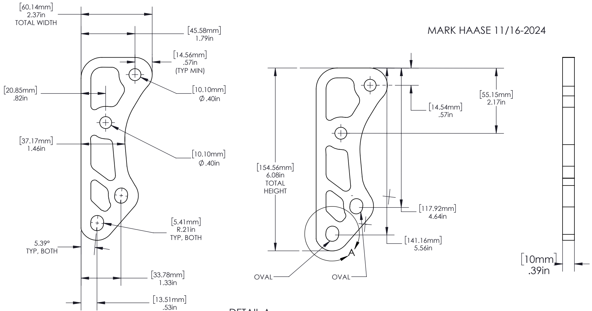
DETAIL A SCALE 1 : 1 OVAL DIMS
