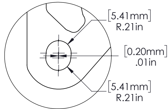
DETAIL A SCALE 1 : 1 OVAL DIMS
